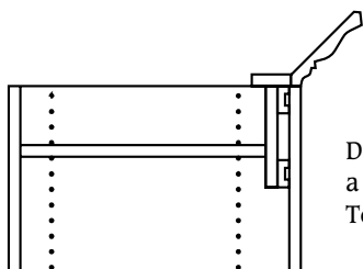
C. Moulding added to Upright Panel. Shown with Header with double-pattern moulding and adjustable shelf used as recessed top.
